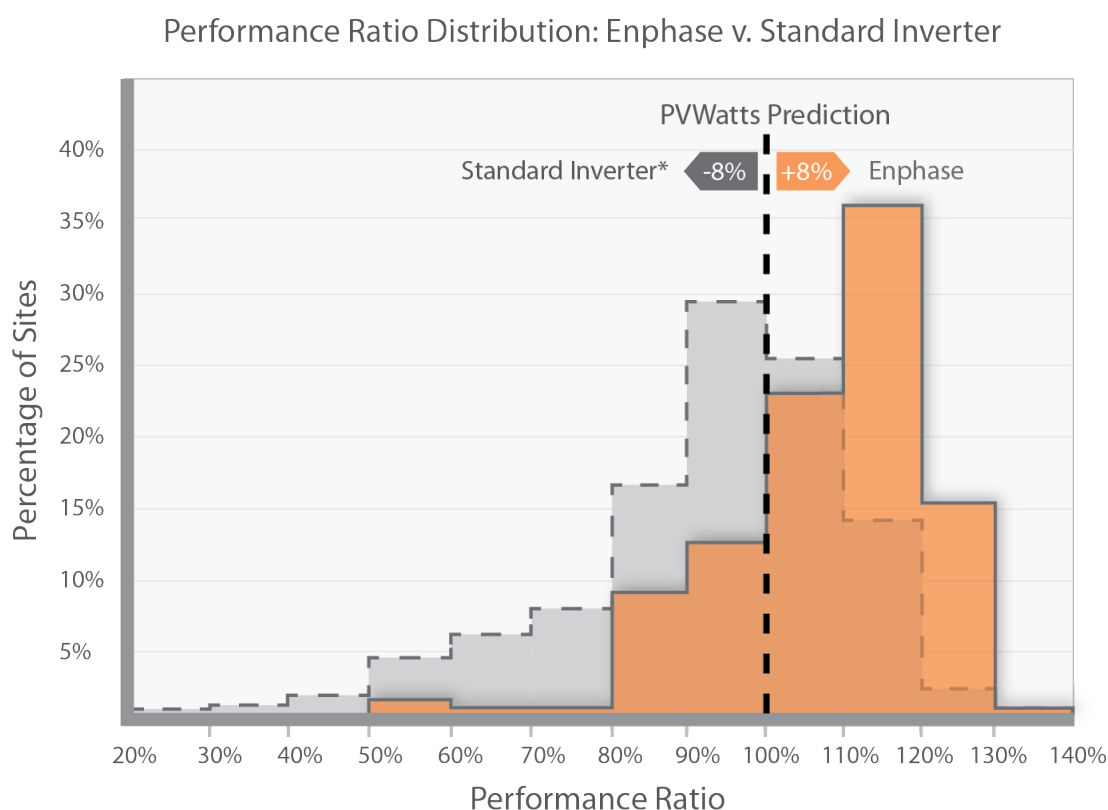
Figure 1 The distributions of performance ratios from Enphase installations and Gostein, et al. are shown in orange and grey, respectively.
