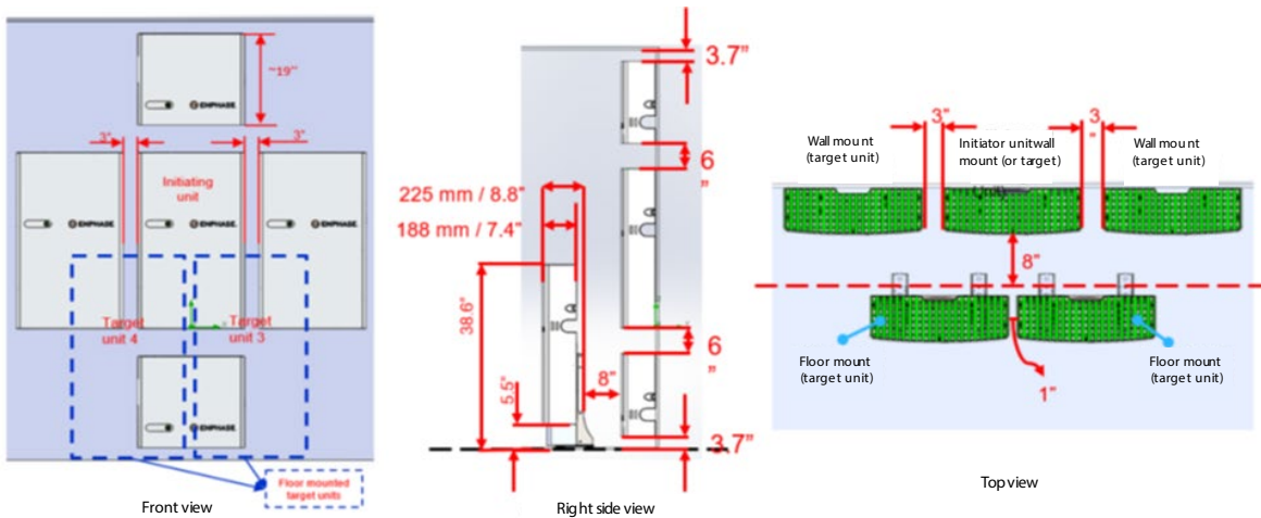
Figure 1: Spacings between the IQ Battery 5P units
