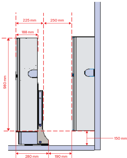
Minimum distance from the floor to the bottom of the unit (for both floor-mounted and wall-mounted)
