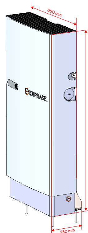
Dimensions of an IQ Battery 5P mounted on a Pedestal Mount
