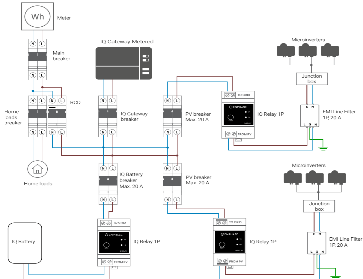
Single-phase system with multiple branches and storage wiring diagram with EMI Line Filter
