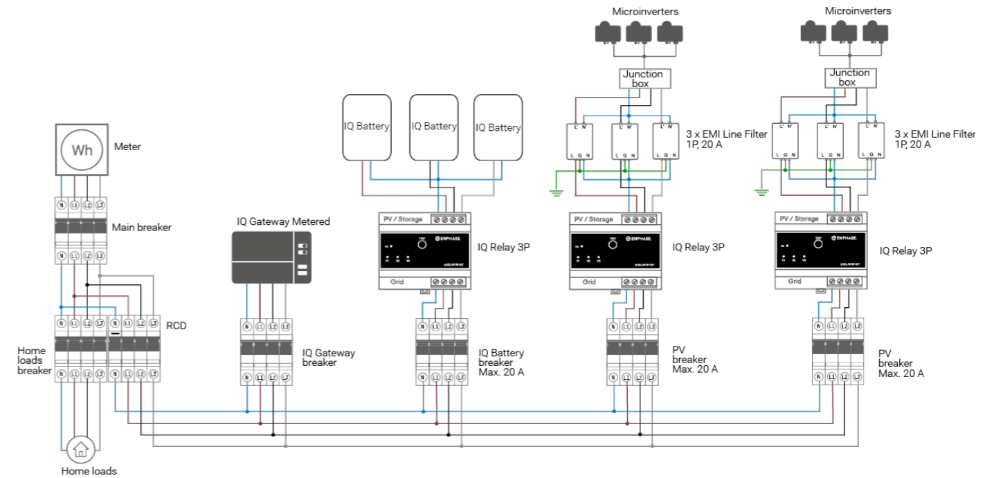
Three-phase system with multiple branches and storage wiring diagram with EMI Line Filter
